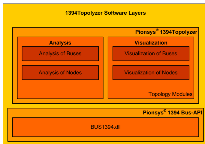
The software layers of the 1394Topolyzer
