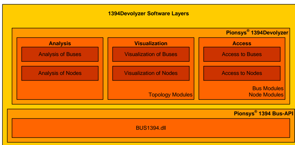
The software layers of the 1394Devolyzer
